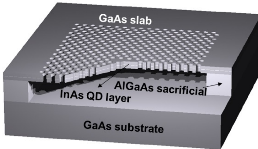
Fig. 3. Schematic of a realistic air-suspended 2D photonic crystal slab made out of a triangular lattice of air holes in Galium Arsenide (GaAs). Embedding quantum dots (QD) in between the slab allows the creation of ‘active’ devices such as lasers.
