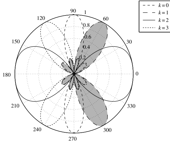
Figure 7.13 The bin \mathcal{R}_k is the set of all paths that arrive roughly in the direction of the main lobes of the beamforming pattern of \mathbf{e}_r(k/L) . Here L_t = 2 and n_r = 4 .
