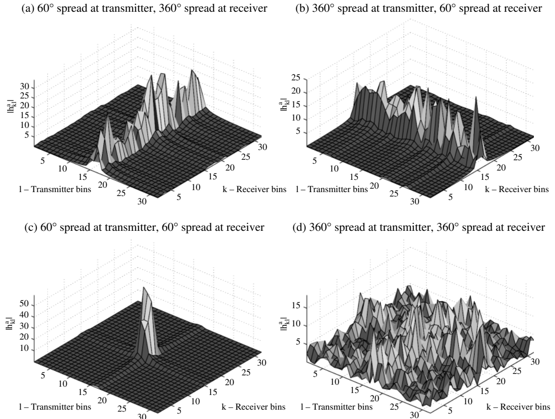
Figure 7.14 Some examples of \mathbf{H}^a . (a) Small angular spread at the transmitter, such as the channel in Figure 7.10(a). (b) Small angular spread at the receiver, such as the channel in Figure 7.10(b). (c) Small angular spreads at both the transmitter and the receiver. (d) Full angular spreads at both the transmitter and the receiver.
