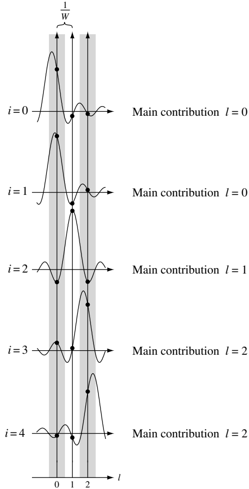
Figure 2.10 Due to the decay of the sinc function, the i th path contributes most significantly to the \ell th tap if its delay falls in the window [\ell/W - 1/(2W), \ell/W + 1/(2W)] .
