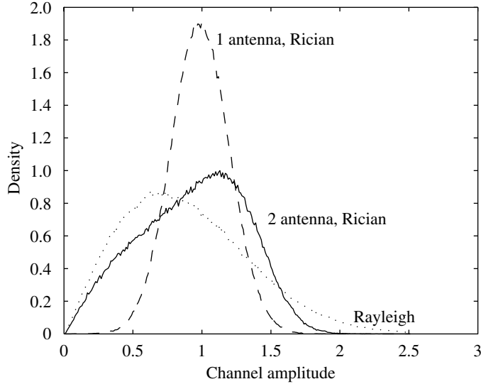
Figure 6.23 Comparison of the distribution of the overall channel gain with and without opportunistic beamforming using two transmit antennas, Rician fading. The Rayleigh distribution is also shown.
