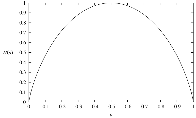
Figure B.3 The binary entropy function.
