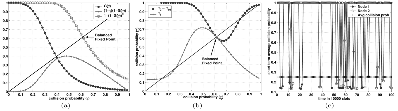
Fig. 1. Example System-I. (a) Balanced fixed point. Plots of G(\gamma) , F(\gamma) = (1-\gamma)(1-G(\gamma)) and 1-(1-G(\gamma))^9 versus the collision probability \gamma ; we also show the “ y = x ” line. (b) Demonstration of unbalanced fixed points. Plots of \gamma_2 = 1 - (1-G(\gamma))^8(1-G(1-(1-G(\gamma))^9)) (the curve drawn with dots and lines) and the function for the fixed point equation for \gamma_1 (see text) using pluses and lines. (c) Snap-shot of short term average collision probability of 2 of the 10 nodes. Also plotted is the average collision probability of the nodes (averaged over all frames and nodes). The 95% confidence interval for the average collision probability lies within 0.7% of the mean value.
