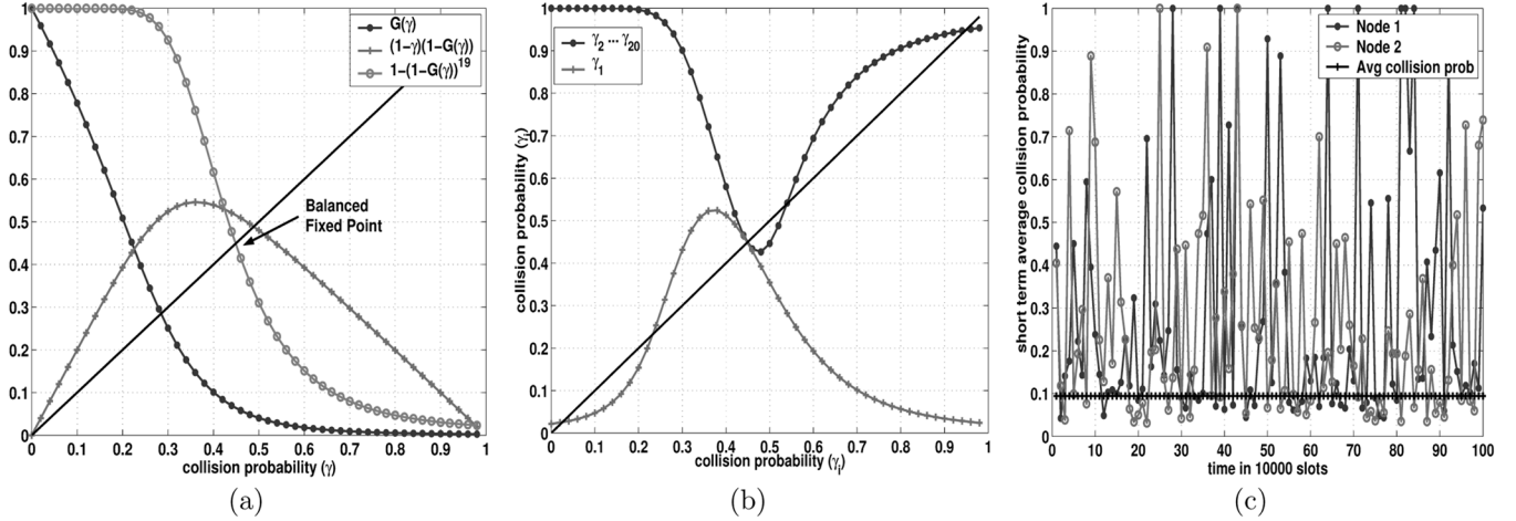
Fig. 2. Example System-II. (a) The balanced fixed point. Plots of G(\gamma) , F(\gamma) = (1 - \gamma)(1 - G(\gamma)) and 1 - (1 - G(\gamma))^{19} versus the collision probability \gamma ; the line “ y = x ” is also shown. Notice that the function F is not one-to-one. (b) Demonstration of unbalanced fixed points. Plots of \gamma_2 = 1 - (1 - G(\gamma))^{18} (the curve drawn with dots and lines) and the function for the fixed point equation for \gamma_1 (see text) using pluses and lines. (c) Snap-shot of short term average collision probability of 2 of the 20 nodes. The average collision probability is also plotted in the figure (averaged over all slots and nodes). The 95% confidence interval for the average collision rate lies within 0.7% of the mean value.
