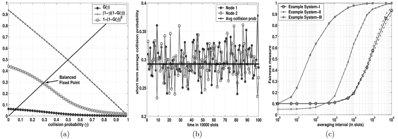
Fig. 3. Example System-III: (a) Plots of G(\gamma) , F(\gamma) = (1-\gamma)(1-G(\gamma)) and 1-(1-G(\gamma))^9 versus the collision probability \gamma ; the line “ y = x ” is also shown. (b) Snap-shot of short term average collision probability of 2 of the 10 nodes. Also plotted is the average collision probability obtained by the nodes. The 95% confidence interval of the average collision rate lies within 0.2% of the mean value. (c) Throughput fairness index of Example III compared with Examples I and II, plotted against the number of slots used to measure throughput. The dotted lines mark the 95% confidence interval for all the three example systems.
