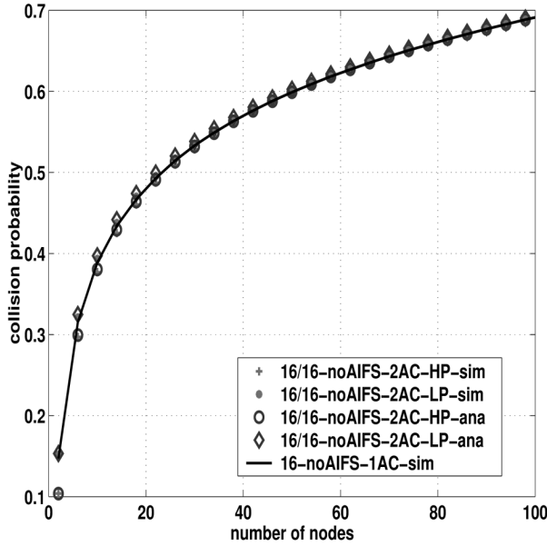
Fig. 7. Collision probability of high priority AC (HP) and low priority AC (LP) in a system of nodes with two ACs. Both simulation (sim) and analysis (ana) are plotted. The backoff parameters of both the ACs (in all the nodes) are identical with b_0 = 16 and AIFS = DIFS. Also plotted is the collision probability (obtained from simulation) for single AC per node case with same backoff parameters and twice the number of nodes. In all the cases p = 2 and K = 7 . For the simulation results, the 95% confidence interval lies within 1% of the mean value.
